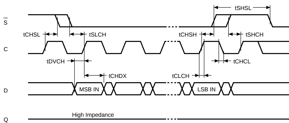
Figure 15. Serial Input Timing
