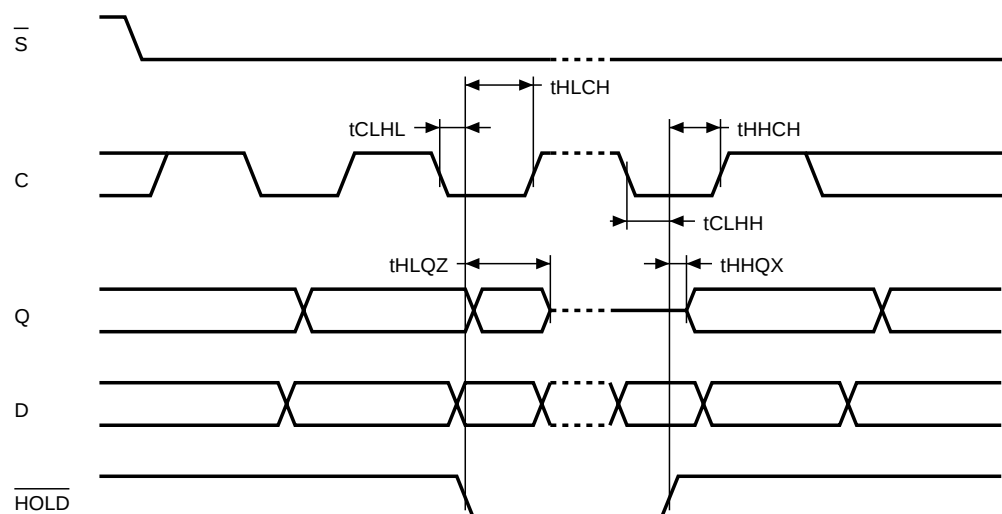
Figure 16. Hold Timing
